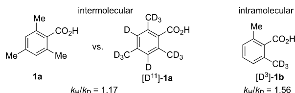
Scheme 6. Kinetic isotope effects.
